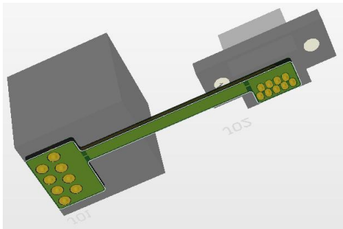
Figure 2 : compatibleCable 4SpW internal flexible PCB
